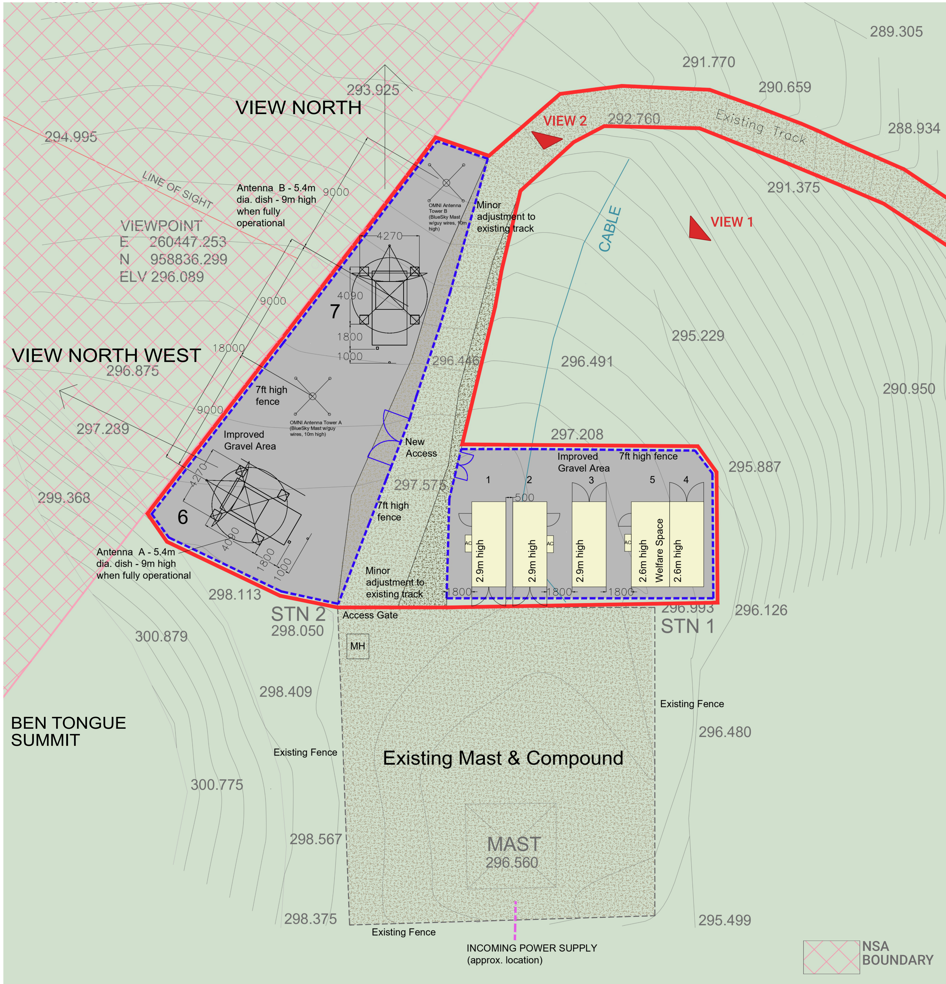
ANTENNA PARK LAYOUT
